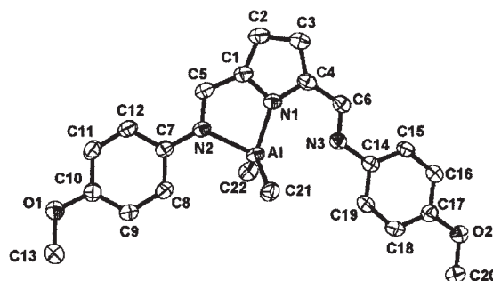
Fig. 1. Molecular structure of 2a with the numbering scheme. Hydrogen atoms are omitted for clarity.
