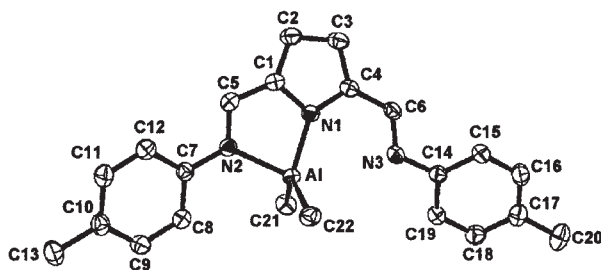
Fig. 2. Molecular structure of 2b with the numbering scheme. Hydrogen atoms are omitted for clarity.
