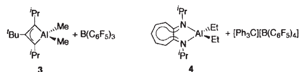
Fig. 3. Aluminum ethylene polymerization catalyst systems.
